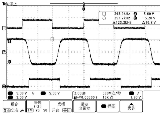
图2. ASRS3222E TIN to TOut to ROut (loopback to Rx with 1000pF load) at 250kbps waveform
