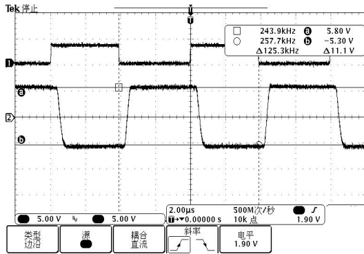
图 1. ASRS3222E T IN to T Out (no load) at 250kbps waveform
